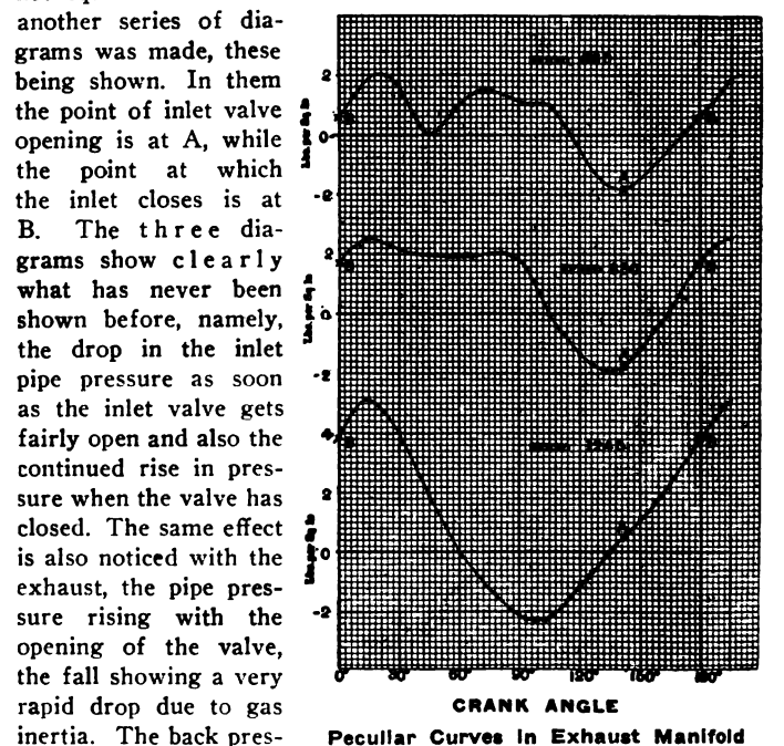
Peculiar Curves in Exhaust Manifold
